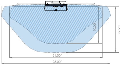
monitor top (shown from above)
